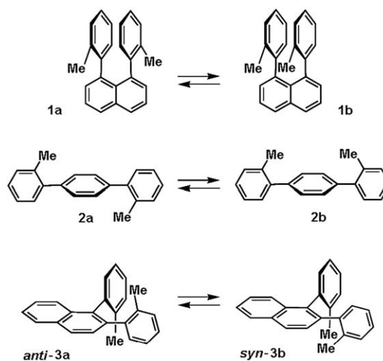
Scheme 1. Atropisomerism in selected teraryls.
