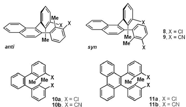
Figure 1. Anti and syn conformers of teraryls 8 , 9 , 10 , and 11 .
