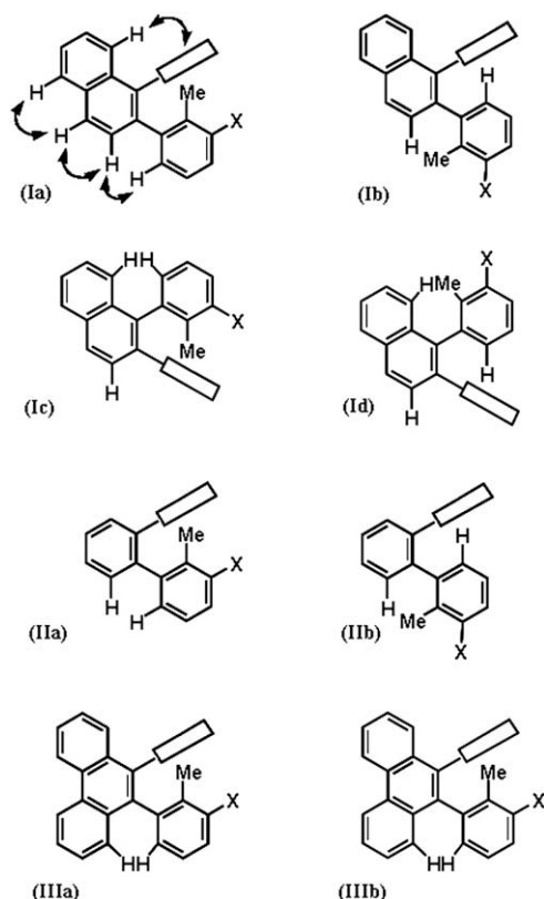
Figure 2. Transition states in the rotational isomerism in ortho -diarylbenzenoids.
