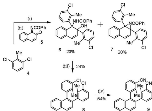
Scheme 2. Synthesis of 1,2-diarylnaphthalenes 8 and 9 . Reagents and conditions: (i) Mg/BrCH 2 CH 2 Br (cat.), THF, reflux, 3 h; (ii) 5 , benzene, reflux, 3 h; rt, 8 h; (iii) Zn, AcOH, 2% aq [H 3 O] + [PtCl 6 ] 2- (cat.), concd HCl, reflux, 16 h; (iv) CuCN, N -methyl-2-pyrrolidinone, reflux, 32 h.
